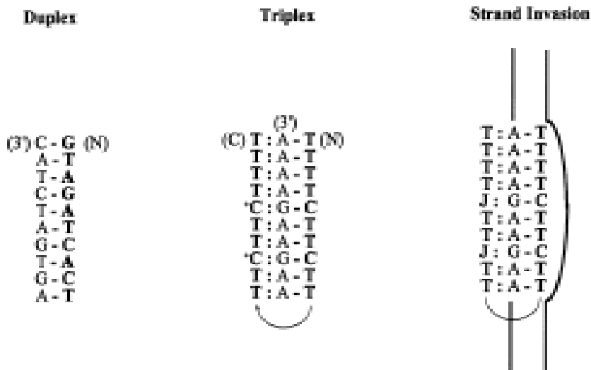
Figure 2. Schematic representation of a PNA-DNA duplex in the antiparallel mode (3'-end of the DNA facing the amino-terminal of the PNA), a 2PNA/DNA triplex in the preferred binding mode with antiparallel Watson-Crick strand and parallel Hoogsteen strand a linker of a bis-PNA is indicated), and a triplex strand invasion complex using a bis-PNA with J-bases in the Hoogsteen strand. PNAs are shown in bold. Watson-Crick hydrogen bonds are indicated by '-', while Hoogsteen Crick hydrogen bonds are indicated by ':'.
